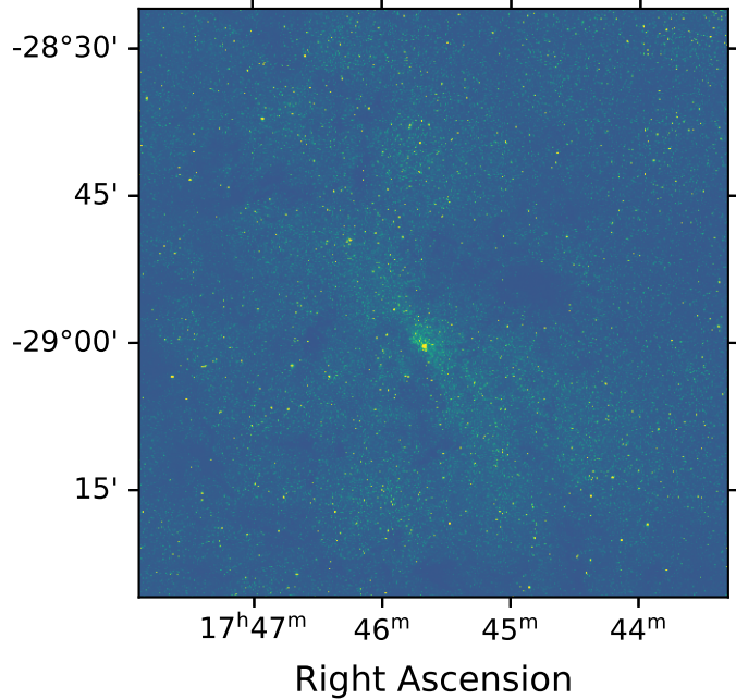
2MASS K-band
